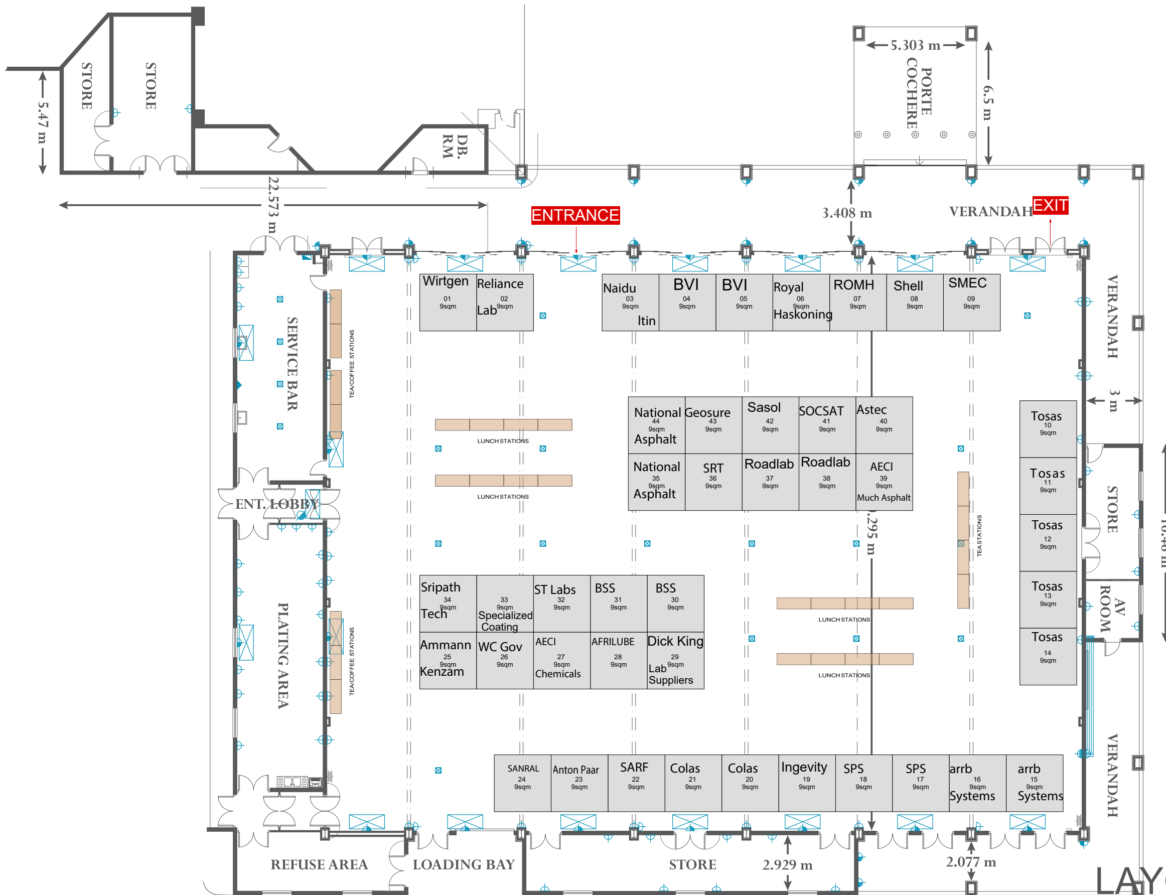
Floor Plan Scale 1: 200
